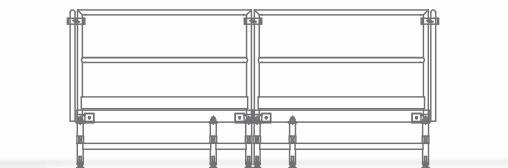
Side C – Elevation View 36" high ADA-Compliant Ramp
